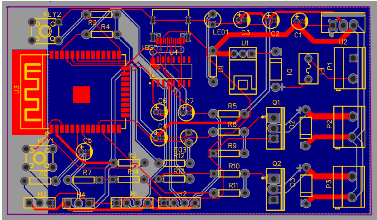
Figure 3: Top Layer PCB Layout
